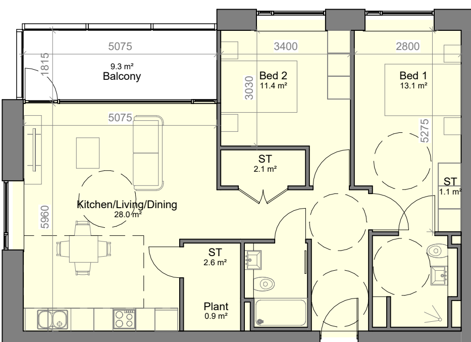
2B4P-TYPE A UD
