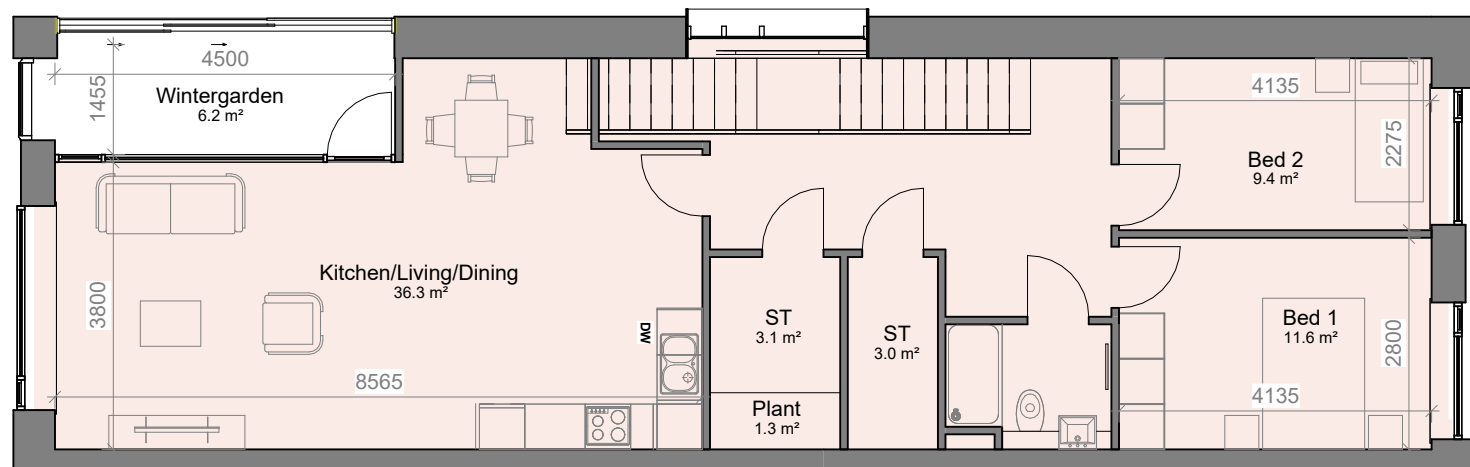
2B4P-TYPE G OD (Own Door)
