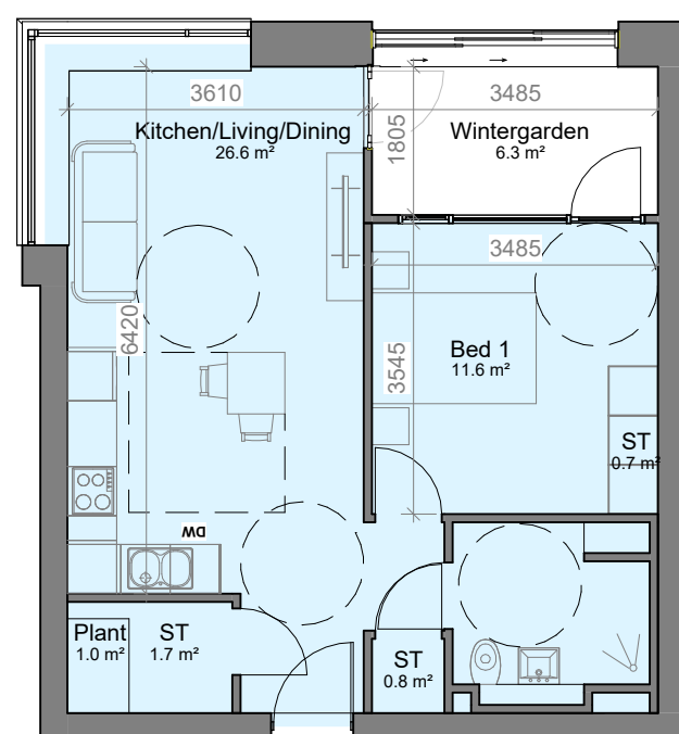
1B2P-TYPE A UD
