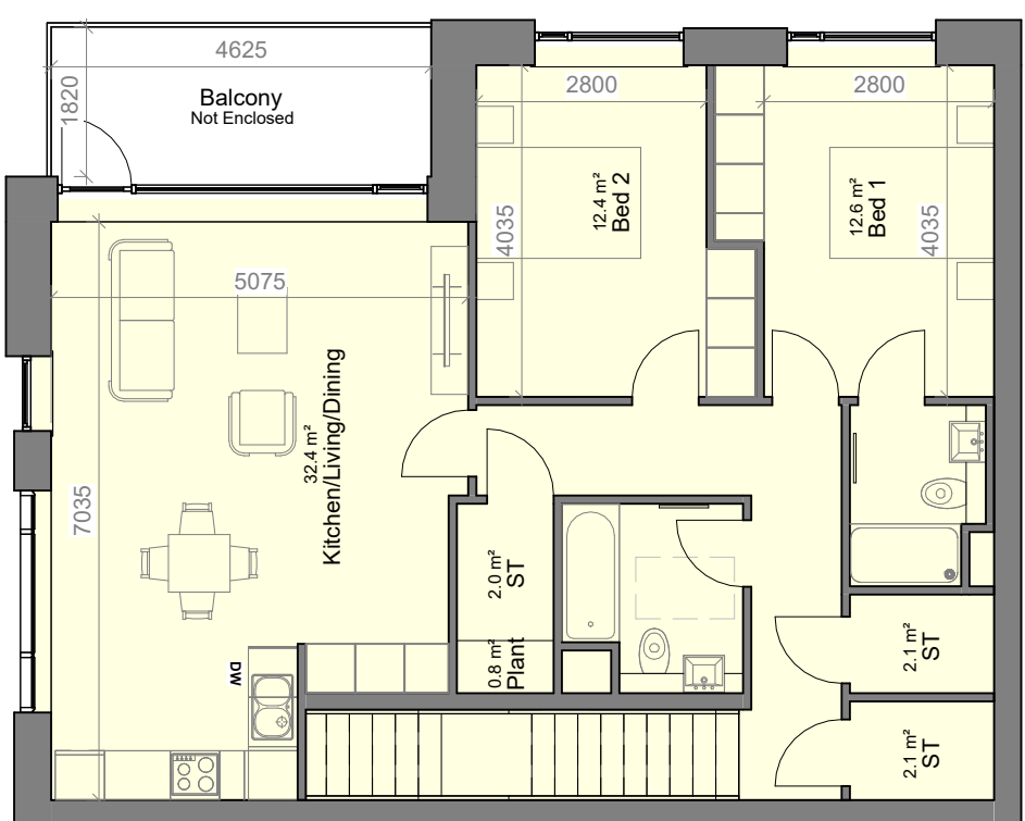
2B4P-TYPE D OD (Own Door)
